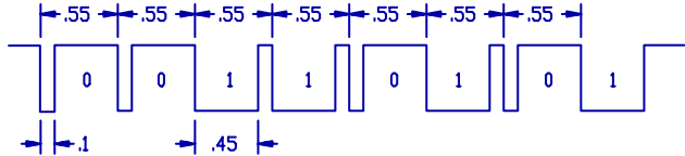
Figure 3. Data Jack Format
