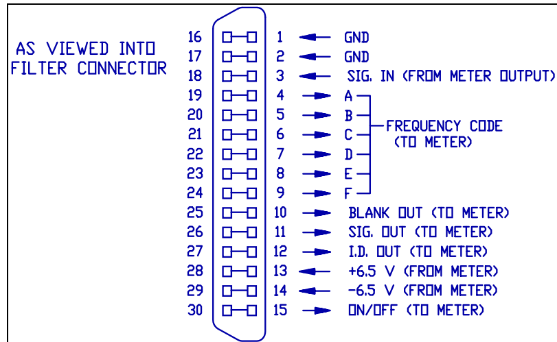
Figure 22. OB-300M External Filter Connector (Located on Top of Filter)
