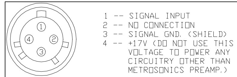
Figure 11 Meter Electrical Input (Direct)
