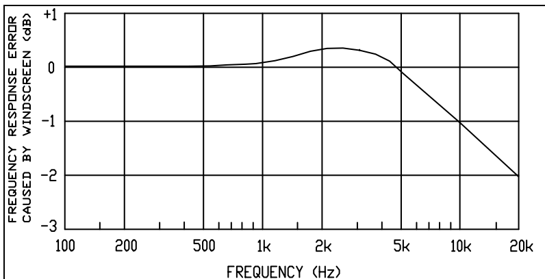
Figure 7. Acoustic Effect of WS-7 Windscreen
