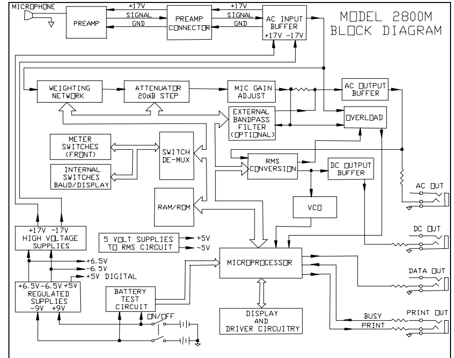
Figure 9. Block Diagram of the Model 2800M
