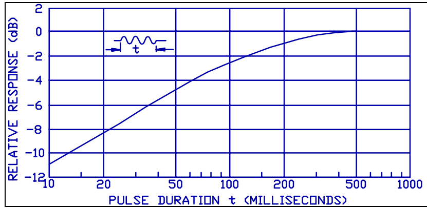
Figure 15 FAST Response
