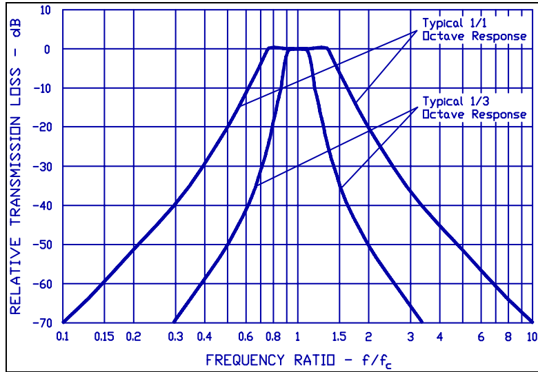
Figure 23. Typical OB-300M Filter Response
