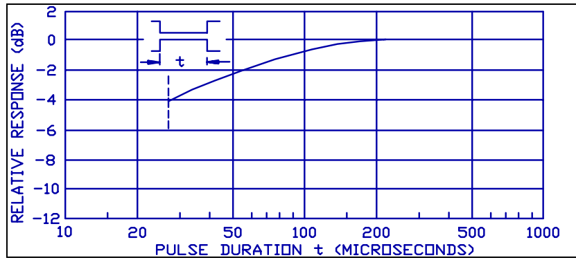
Figure 16 PEAK Response
