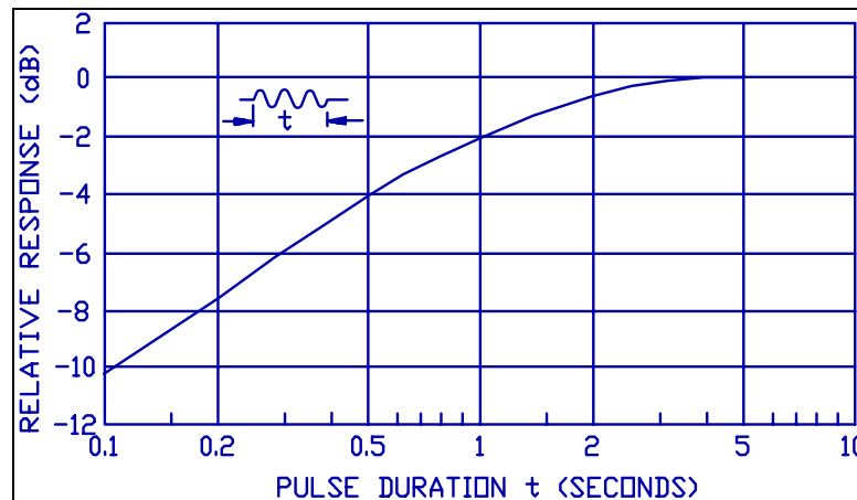
Figure 14. SLOW Response
