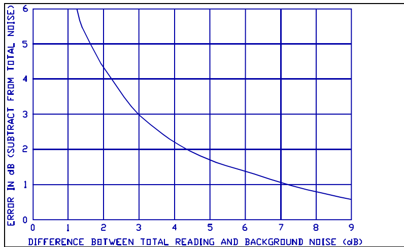
Figure 6 Effect of Background on Measurement
