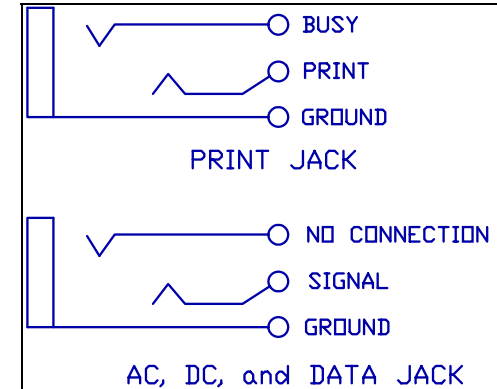
Figure 2. Output Jack Connections
