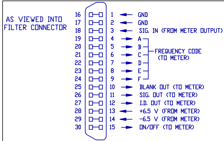
Figure 19 OB-100M External Filter Connector (Located on top of filter)
