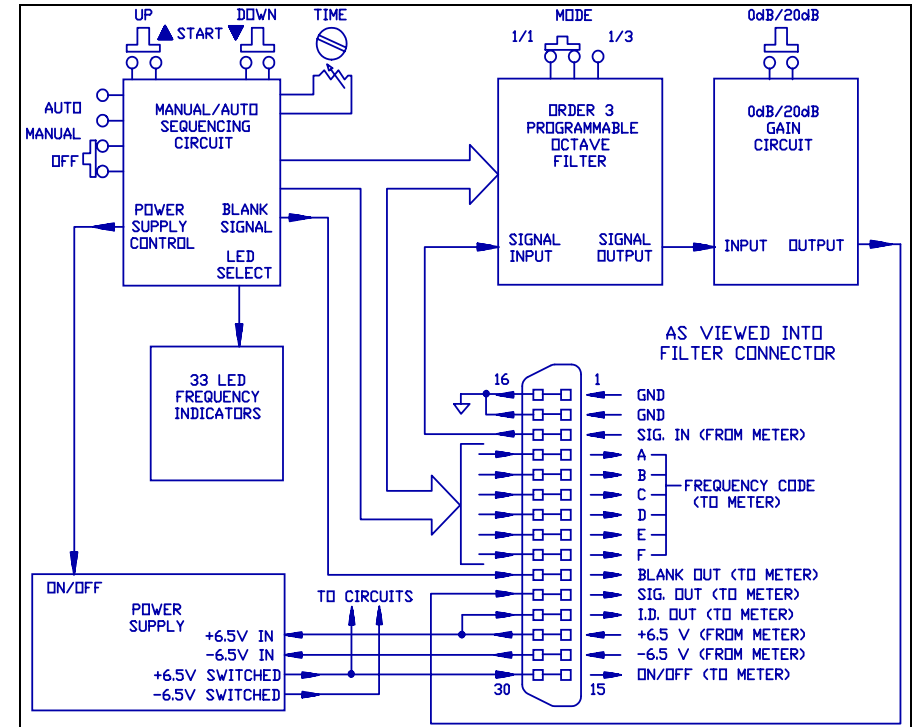
Figure 24. Block Diagram of Model OB-300M
