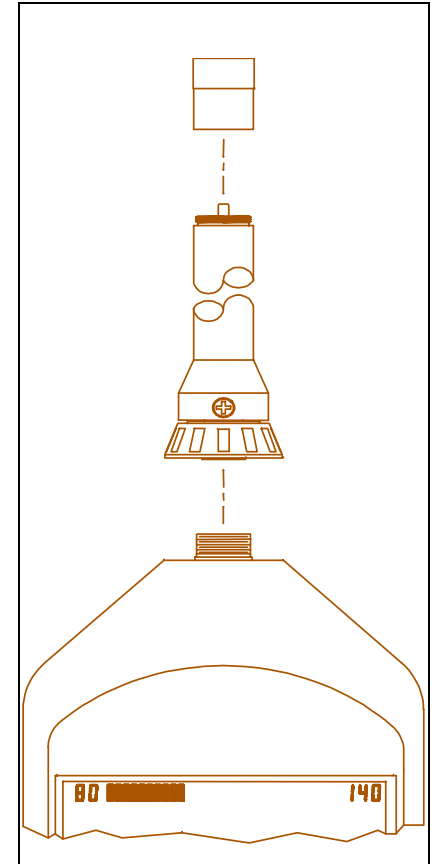
Figure 1 Mic/Preamp Assembly
