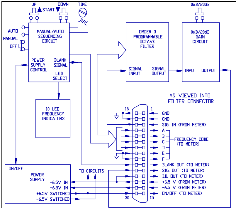
Figure 21. Block Diagram Model OB-100 Octave Filter
