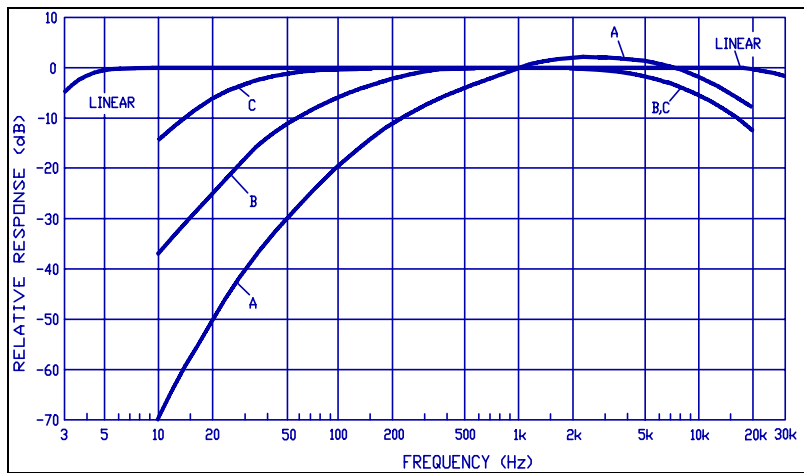
Figure 12 Weighting Characteristics
