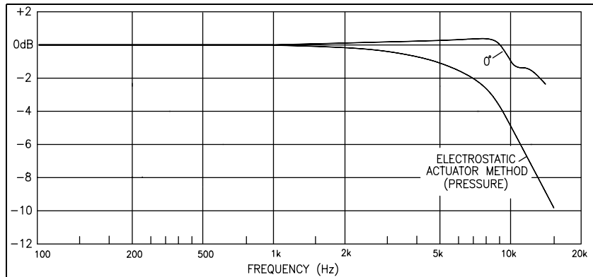
Figure 10. Typical Frequency Response for the Model QE7052 0.5 Inch Microphone
