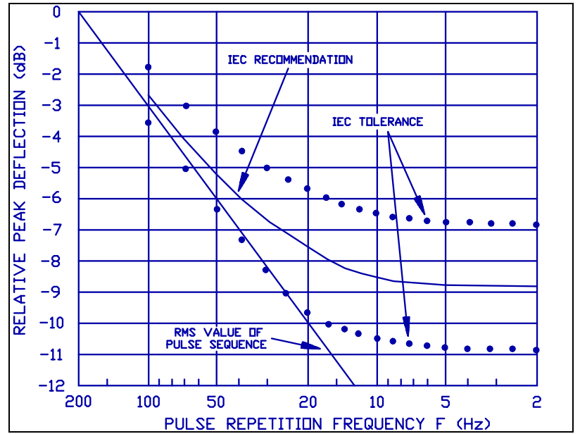
Figure 18 IMPULSE Response to Repeated Impulses
