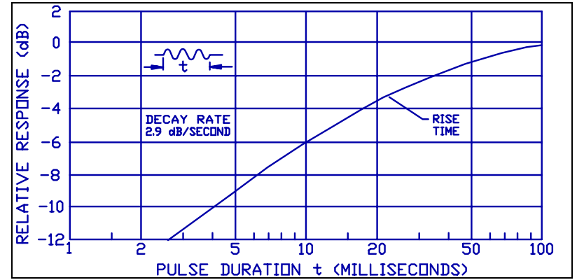
Figure 17 IMPULSE Response
