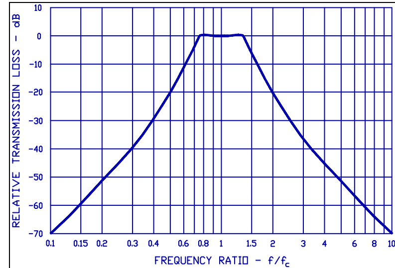
Figure 20. Typical OB-100M Filter Response
